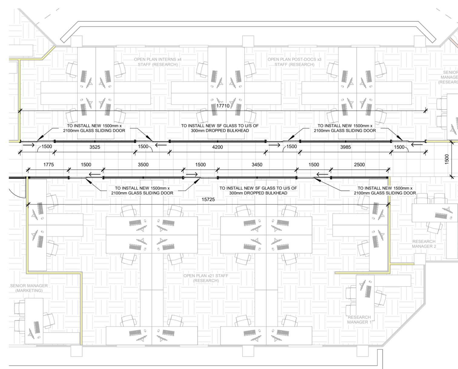
2. 3rd FLOOR PROPOSED LAYOUT - RESEARCH OPEN PLAN AREA (ALTERATIONS)
