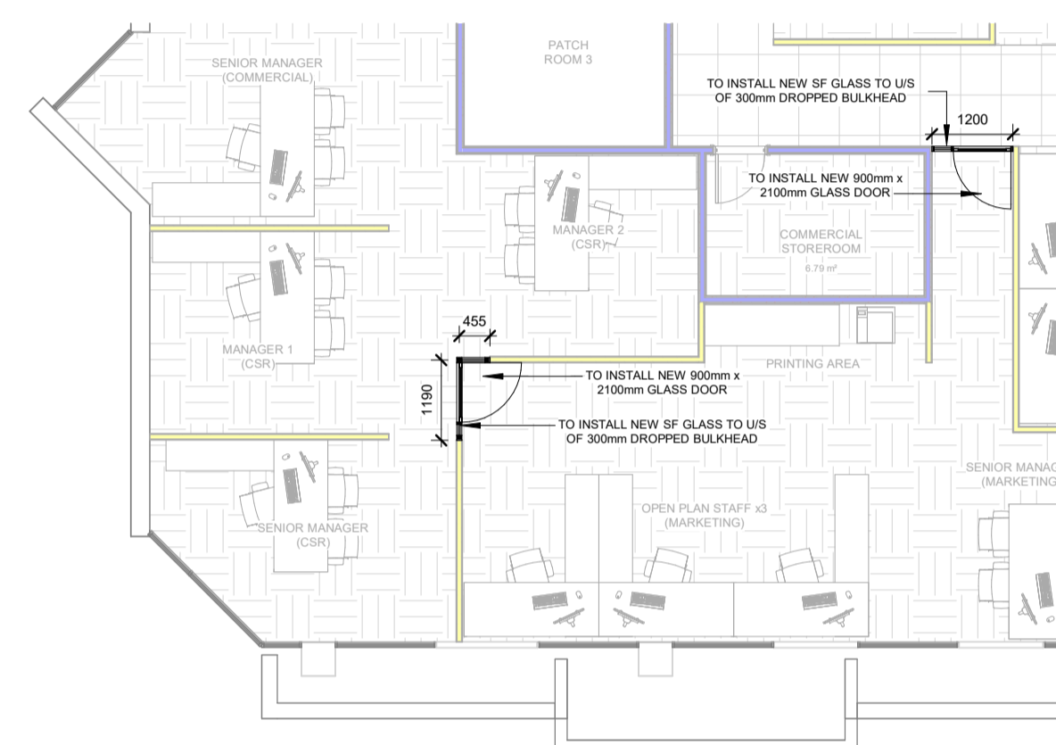
3. 3rd FLOOR PROPOSED LAYOUT - MARKETING AREA (ALTERATIONS)
