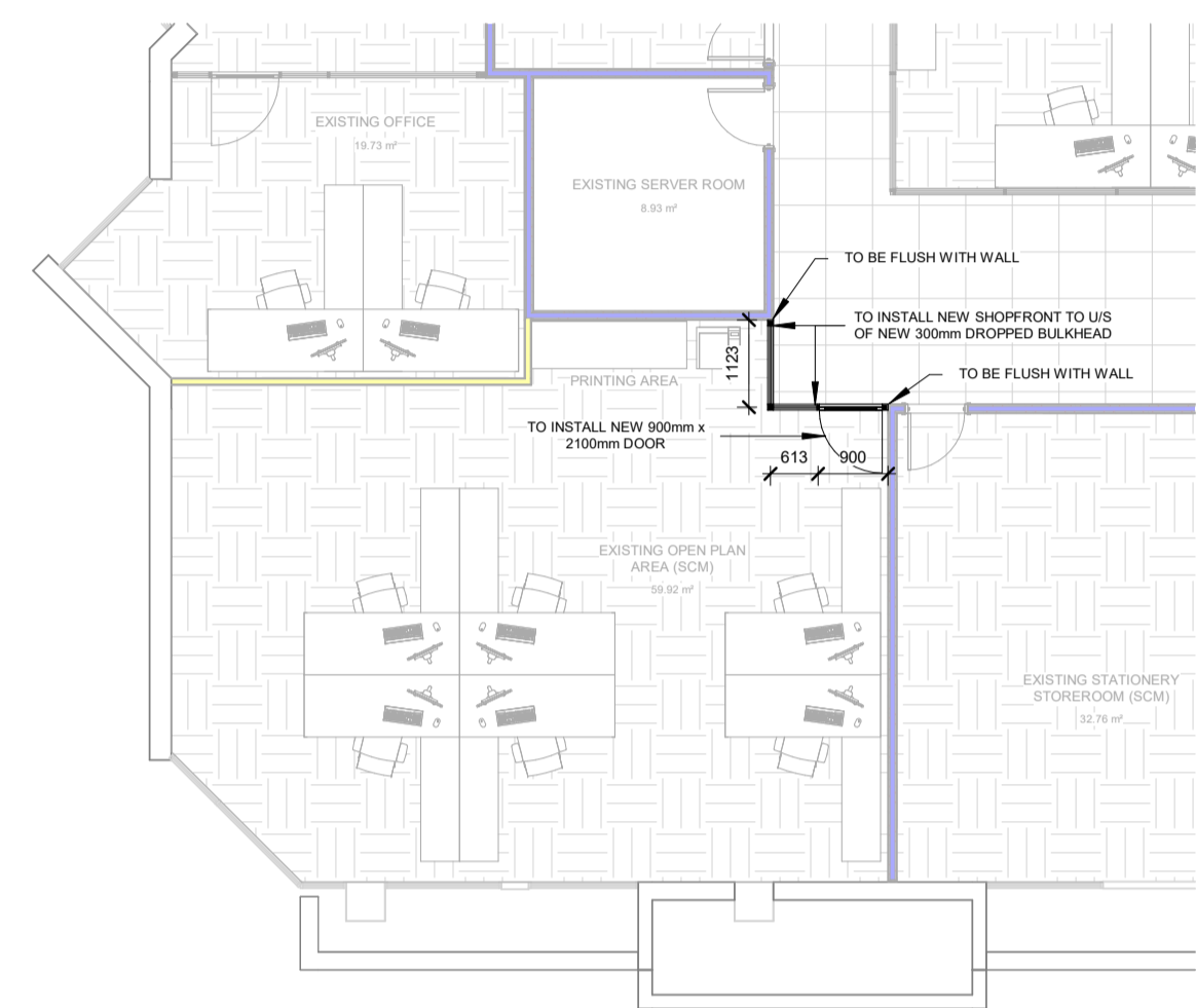
1. 2nd FLOOR PROPOSED LAYOUT - SCM OPEN PLAN AREA (ALTERATIONS)
